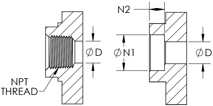
SCREWED END SOCKET WELD END
